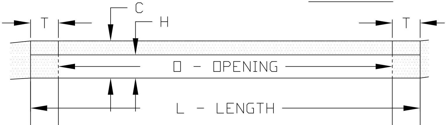
SECTION VIEW
